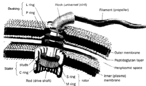
Drawing of a bacterial flagellum showing the filament, hook, and the motor imbedded in the inner and outer cell membranes and the cell wall. From Voet and Voet, Biochemistry , 2d ed. © 1995 John Wiley
